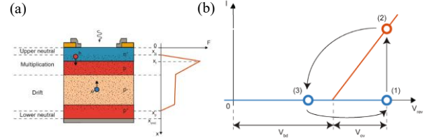
Fig. 1. a) Basic Structure of a SPAD, with corresponding electric field F . b) I-V characteristic of a SPAD; V_{\text{rev}} is the reverse bias; V_{\text{bd}} is the breakdown voltage, and V_{\text{ov}} is the overvoltage [2].
